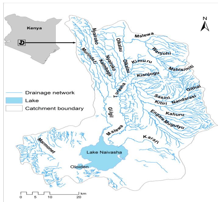
Figure 2.4: Major inflows of Lake Naivasha and catchment boundary
